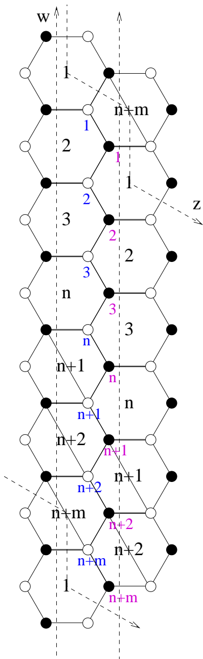
Figure 12: The generic dimer for Y^{p,q} , from [18].
