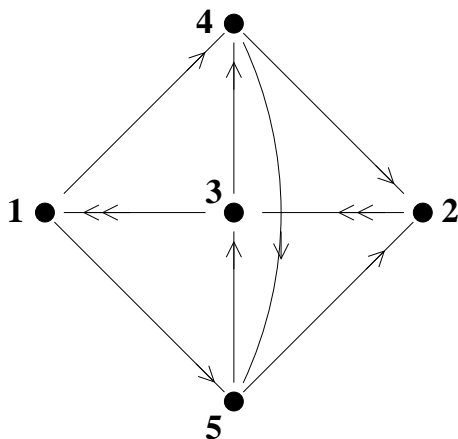
Figure 3: Quiver diagram for the dP_2 theory.
