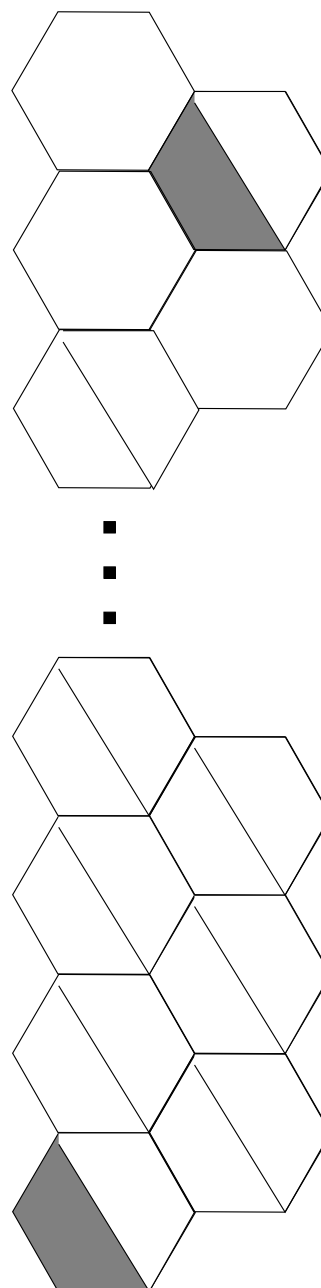
Figure 13: The dimer for Y^{p,1} .
