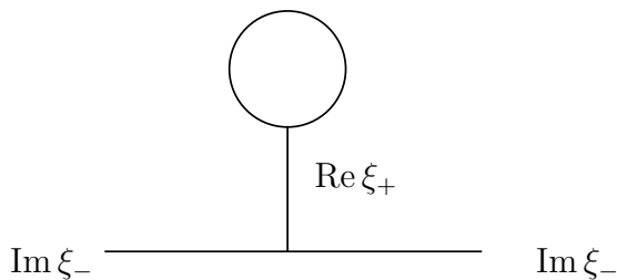
Figure 1: Schematic tadpole contribution to the \text{Im } \xi_- two point function. Both bosons and fermions run in the loop.
