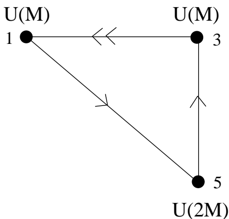
Figure 3: Quiver diagram for the dP_2 theory.
