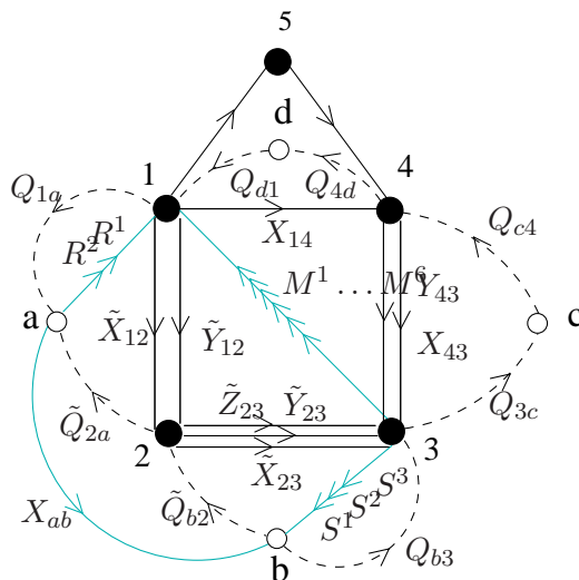
Figure 23: Quiver after Seiberg duality on node 2.
